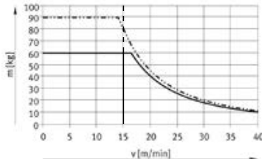
— DFSP-Q-40-R - - - DFSP-Q-50-R
