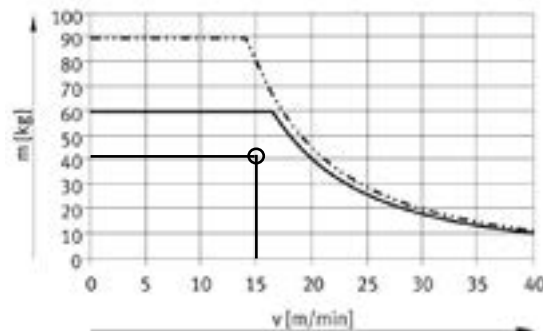
— DFSP-Q-40-R - - - DFSP-Q-50-R
