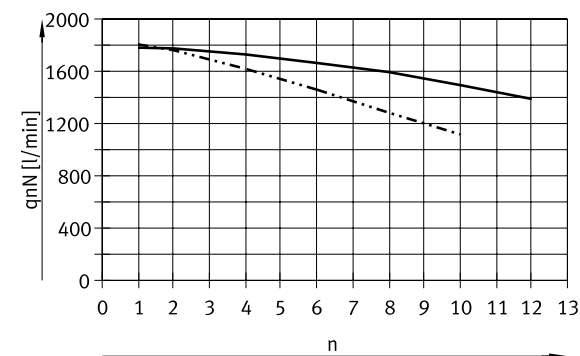
Size 30 – Standard nominal flow rate q_{nN} , with several valves n switched in parallel For 3/2-way valves For 5/2- and 5/3-way valves
