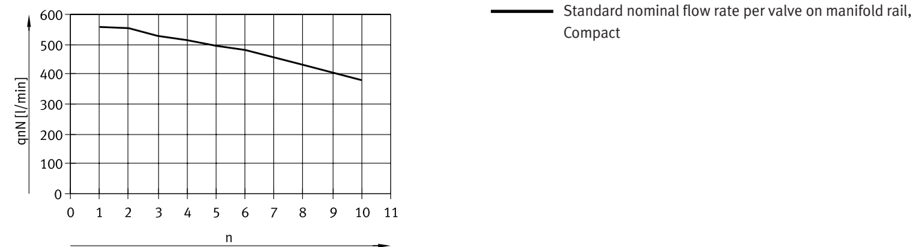
For 5/2-way valves
