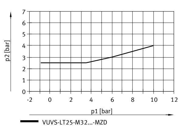
Size 25 – Pilot pressure p2 as a function of working pressure p1 with external pilot air supply For 3/2-way valves For 5/2-way valves, single solenoid
