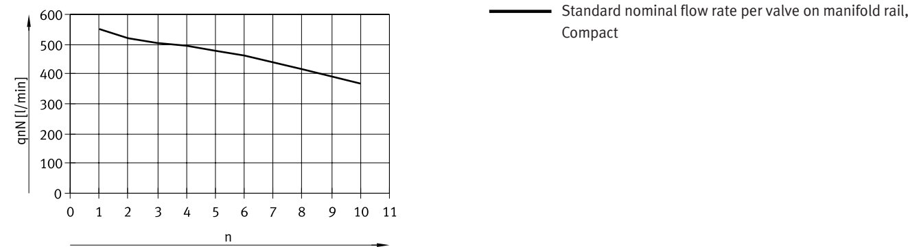
Size 25 – Standard nominal flow rate q_{nN} , with several valves n switched in parallel For 3/2-way valves
